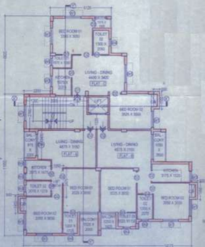
PROPOSED 1st & 2nd FLOOR PLAN. (SCALE: 1:100)
