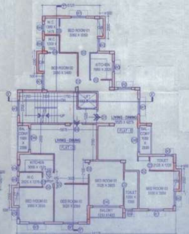
PROPOSED 3rd FLOOR PLAN. (SCALE: 1:100)
